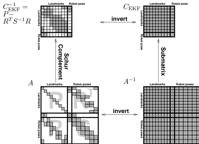
Figure 5. Relation between the LLS information matrix A = \begin{pmatrix} P & R^T \\ R & S \end{pmatrix} which represents all robot poses and the covariance matrix C_{\text{EKF}} used by EKF only representing the actual robot pose. A^{-1} is the covariance matrix corresponding to A . C is derived from A^{-1} as a submatrix removing old robot poses. Accordingly C_{\text{EKF}}^{-1} is the information matrix corresponding to C_{\text{EKF}} . It is derived from A via Schur complement. So on the whole, taking a submatrix of a covariance matrix is equivalent to applying Schur complement to an information matrix.
