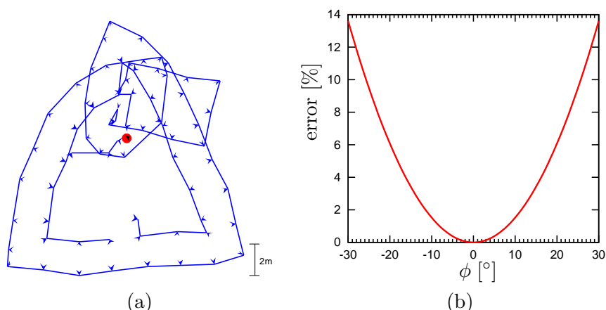
Figure 4. Linearization error: (a) closing the loop with EKF / LLS (b) linearization error of linearized rotation \left| \begin{pmatrix} \cos \phi & \\ & \sin \phi \end{pmatrix} - \begin{pmatrix} 1 & \\ & \phi \end{pmatrix} \right| as a function of angular error \phi
