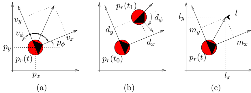
Figure 2. Coordinates describing the robot state p_r = (p_x, p_y, p_\phi)^T and measurements: (a) Continuous odometry measurement: velocity in robot coordinates v_r = (v_x, v_y, v_\phi)^T (b) Discrete odometry measurement: relative movement d_r = (d_x, d_y, d_\phi)^T from p_r(t_0) to p_r(t_1) (c) Landmark measurement: relative position m = (m_x, m_y)^T of landmark at l = (l_x, l_y)^T
