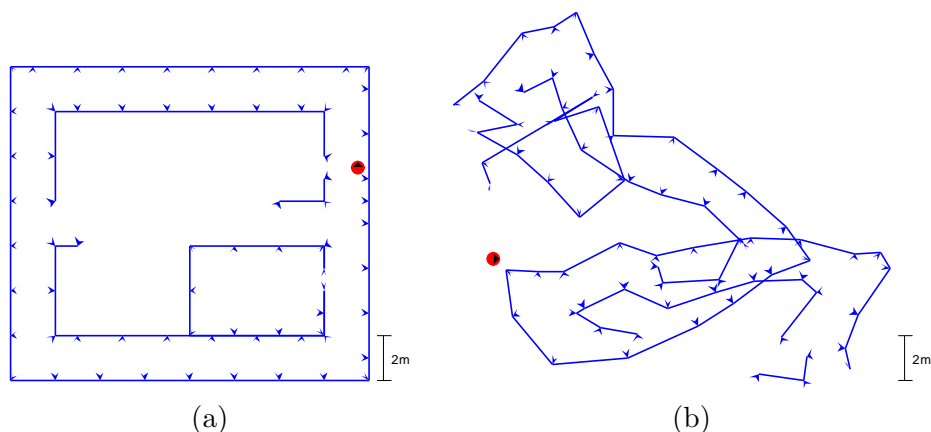
Figure 1. (a) Exact map of the building used as an example. (b) Map derived from raw odometry data. All maps are based on simulations in which the measurements are perturbed by comparatively large artificial noise and bias.
