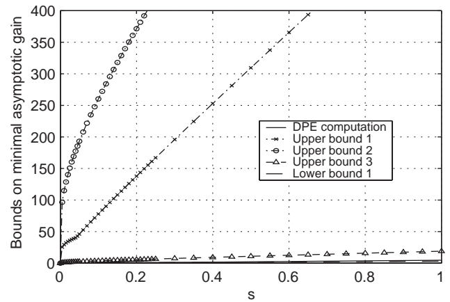
Fig. 2. Comparison of \gamma_\infty obtained by dynamic programming, upper bounds 1–3, and lower bound 1 (Example 3).
