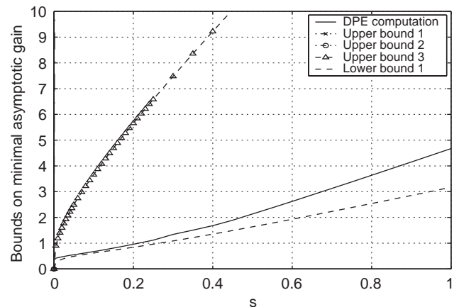
Fig. 3. Enlargement of Fig. 2 illustrating the DPE computation and lower bound (Example 3).
