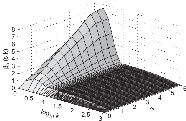
Fig. 4. Approximation of \beta_a (Example 3).
