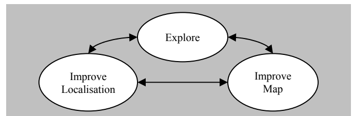
Fig. 1 Exploration States
