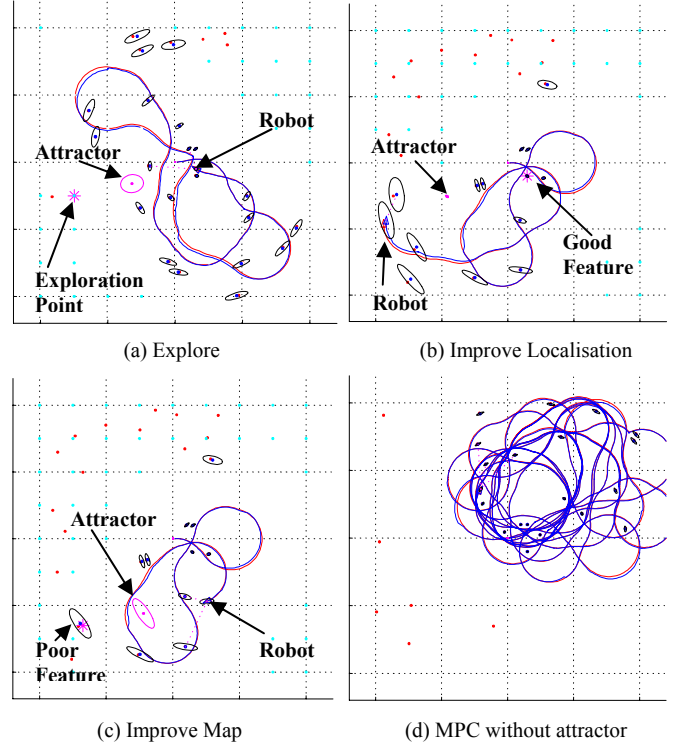
Fig. 2 Robot Exploring with SLAM, MPC and attractor
