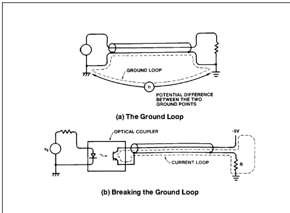
Figure 6.17 – Use of optical coupler
