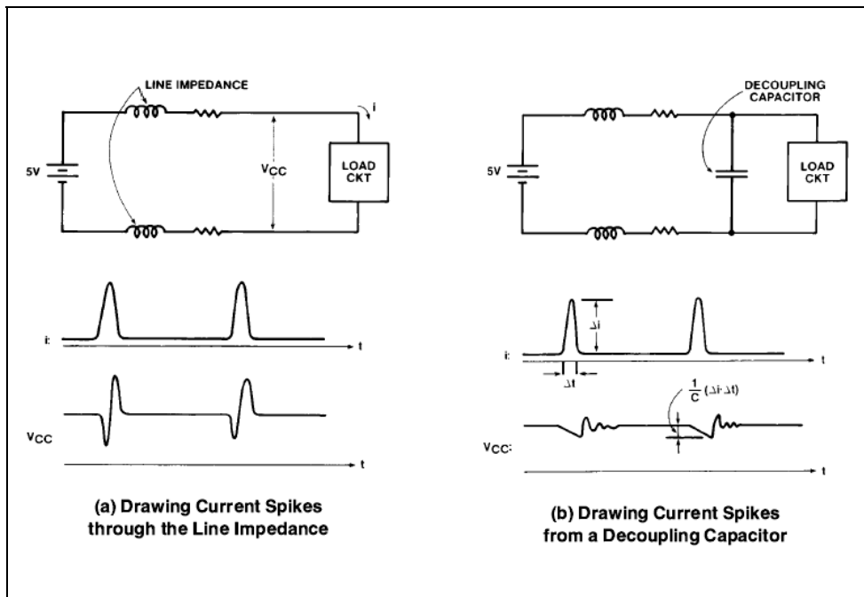
Figure 6.31 – What a decoupling capacitor does
