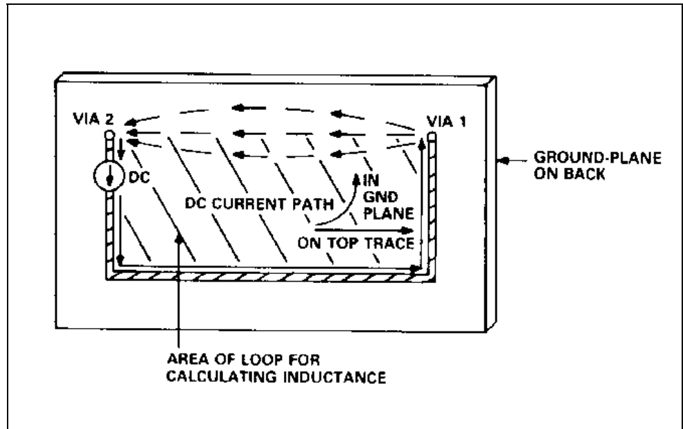
Figure 6.28 – DC current path
