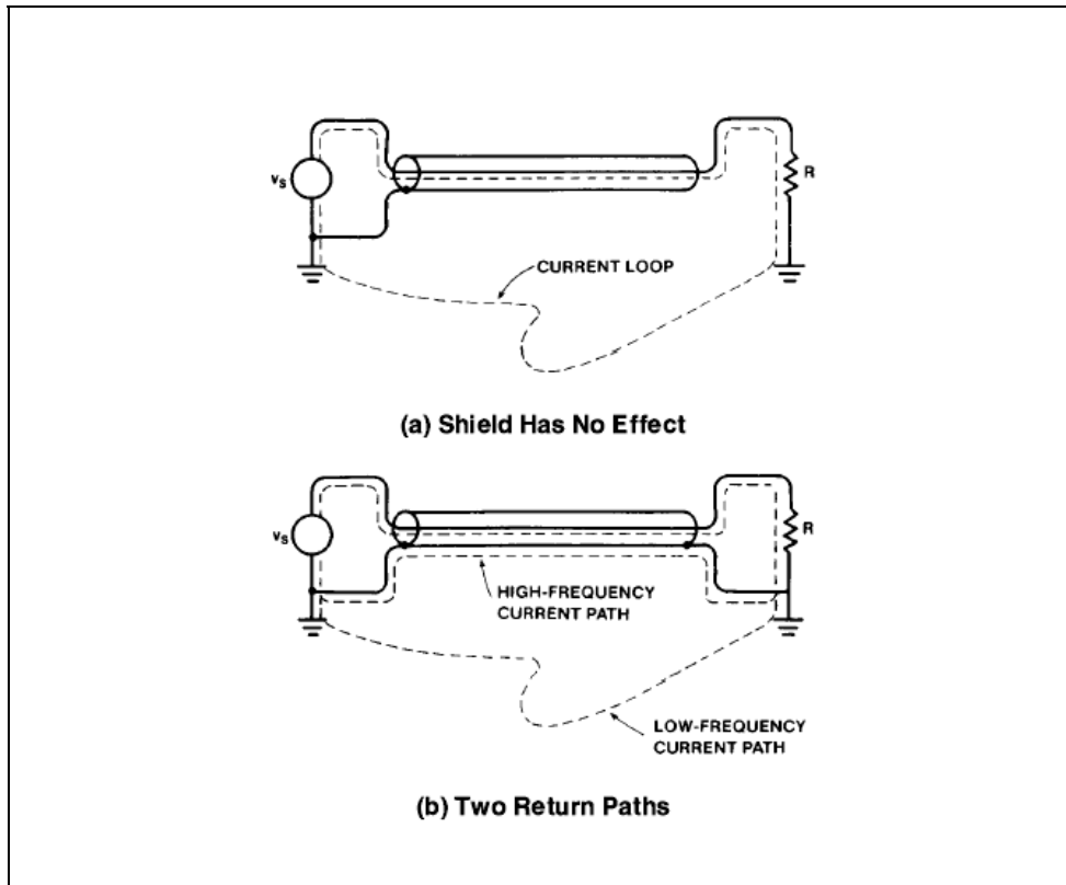
Figure 6.16 – Use of coaxial cable
