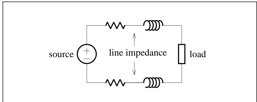
Figure 6.2 – Supply Line Transients
