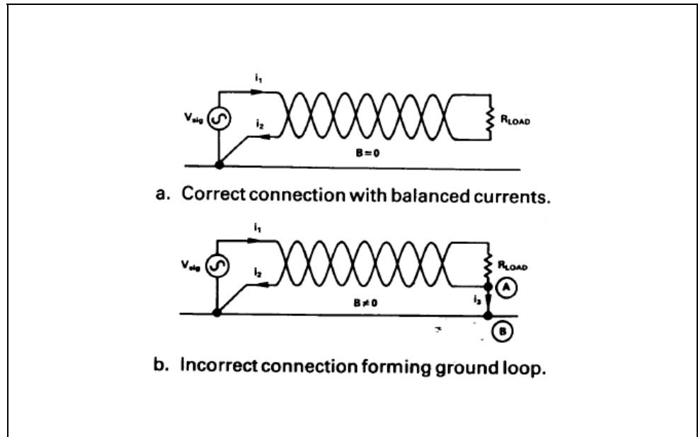
Figure 6.18 – Connections of a twisted pair
