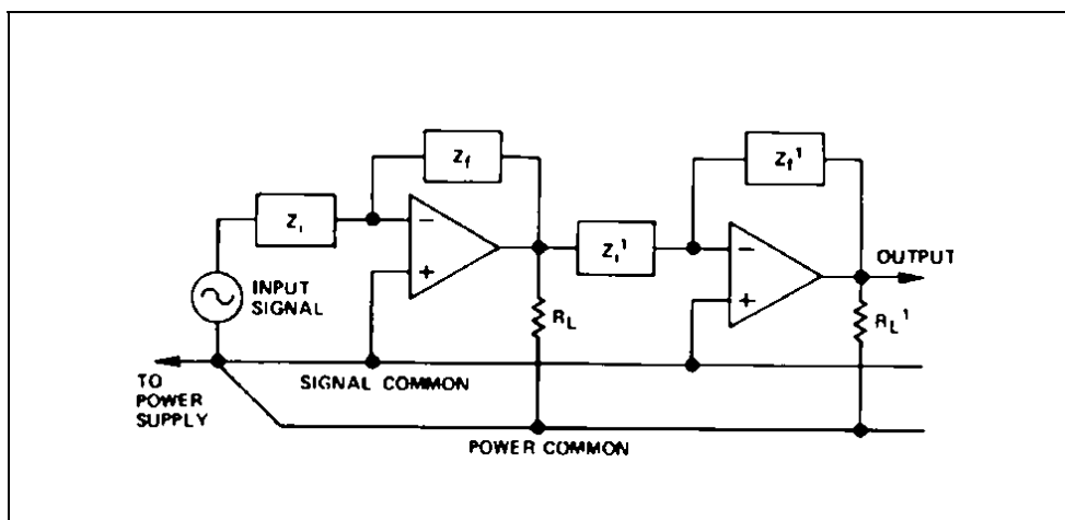
Figure 6.27 – Minimizing common impedance coupling
