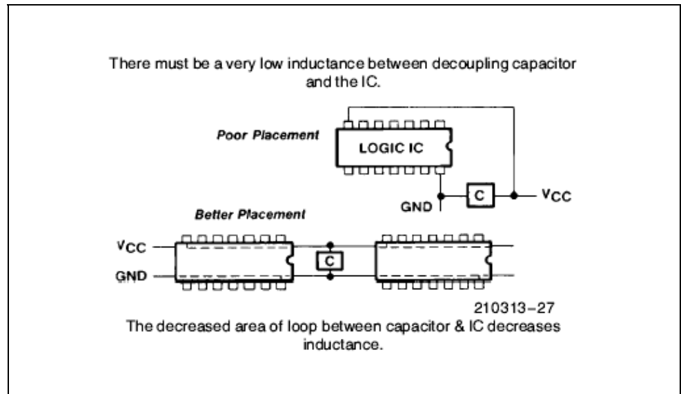
Figure 6.32 – Placement of decoupling capacitors
