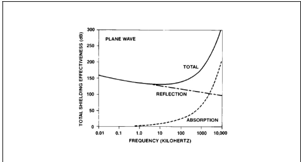
Figure 6.23 – E- and H-field shielding
