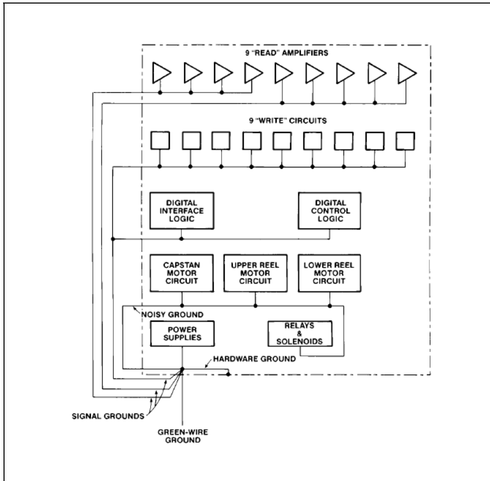
Figure 6.26 – Ground systems in a 9-track digital recorder
