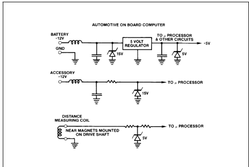
Figure 6.33 – Use of transient suppressors in automotive applications
