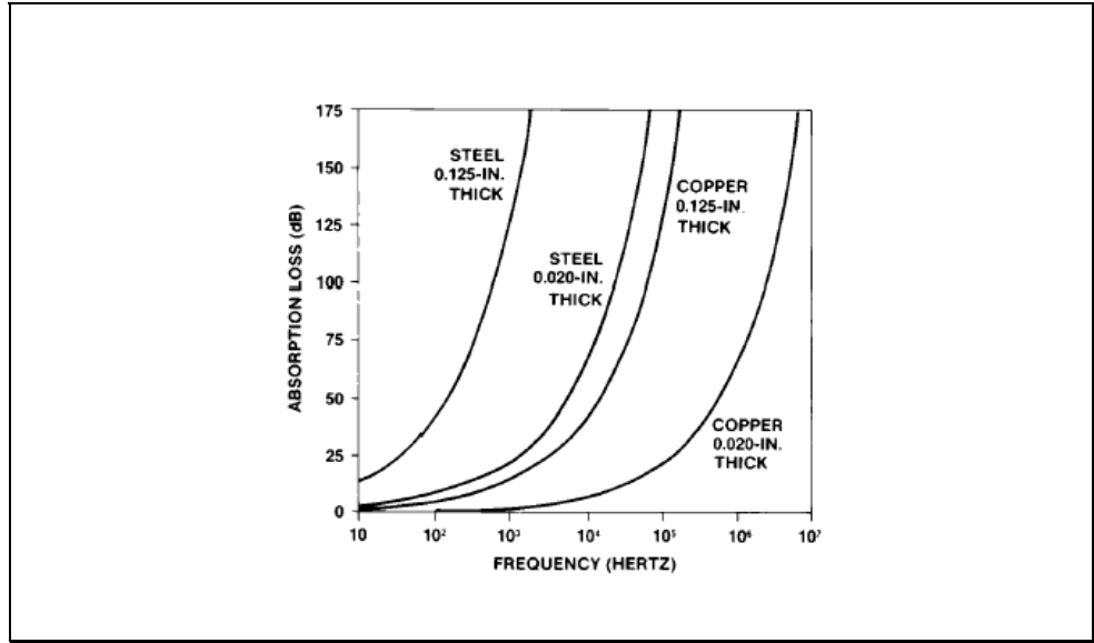
Figure 6.22 – H-field shielding
