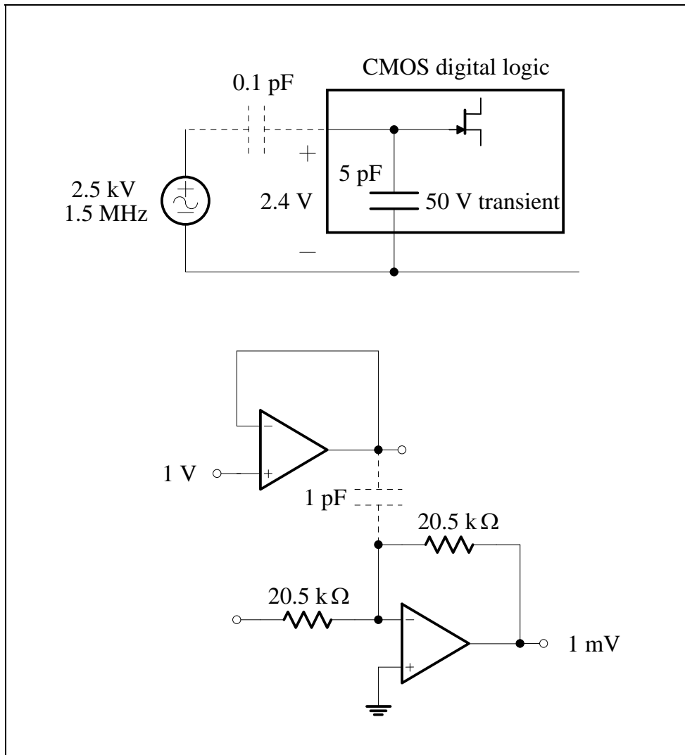
Figure 6.4 – Stray capacitance couples “noise” into other circuits
