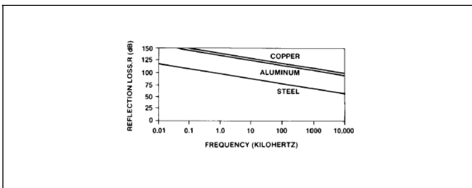
Figure 6.21 – E-field shielding
