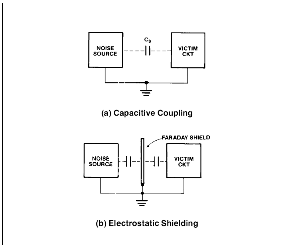
Figure 6.13 – Use of Faraday shield
