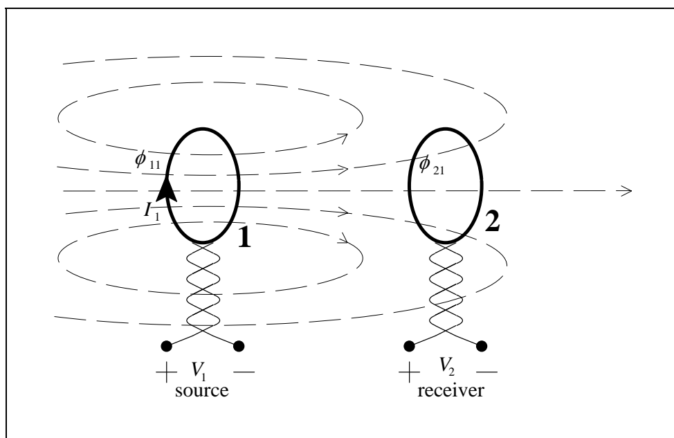
Figure 6.5 – Inductive coupling caused by current loops
