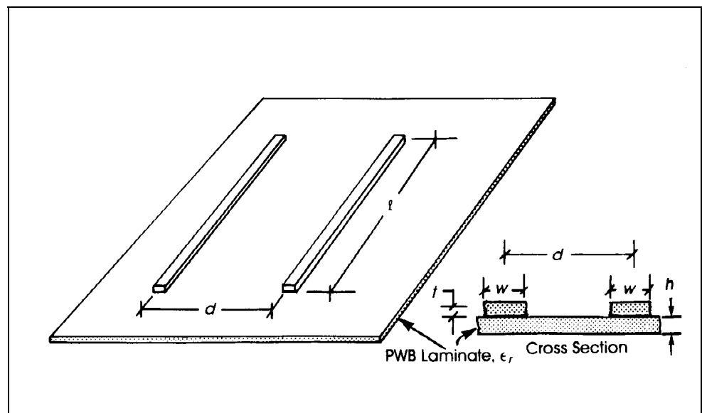
Figure 6.6 – Separate tracks to reduce capacitance
