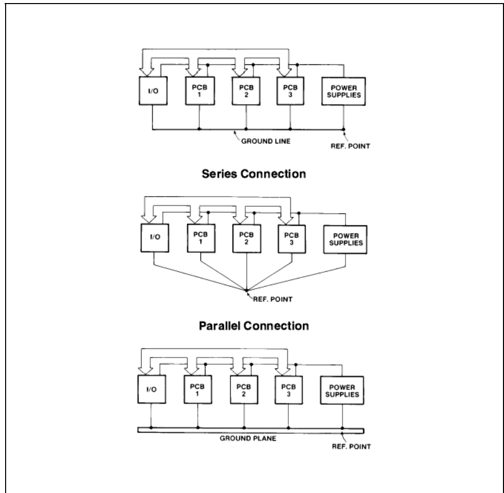
Figure 6.25 – Three ways to wire the grounds
