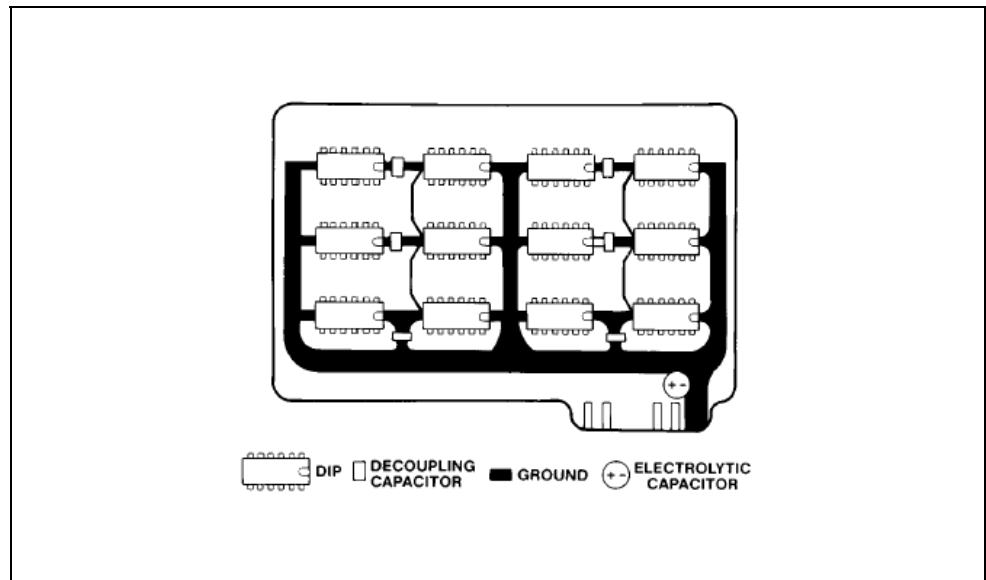
Figure 6.14 – PCB with gridded ground
