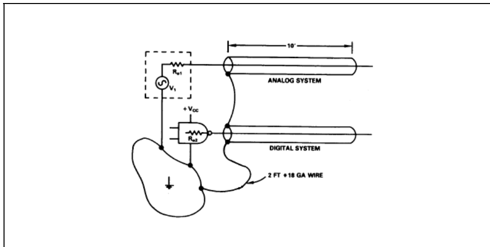
Figure 6.12 – A situation that generates transient shield voltages
