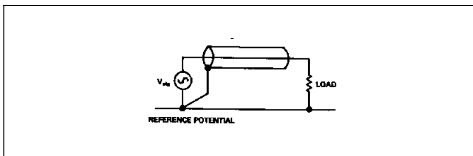
Figure 6.8 – Grounding a cable shield
